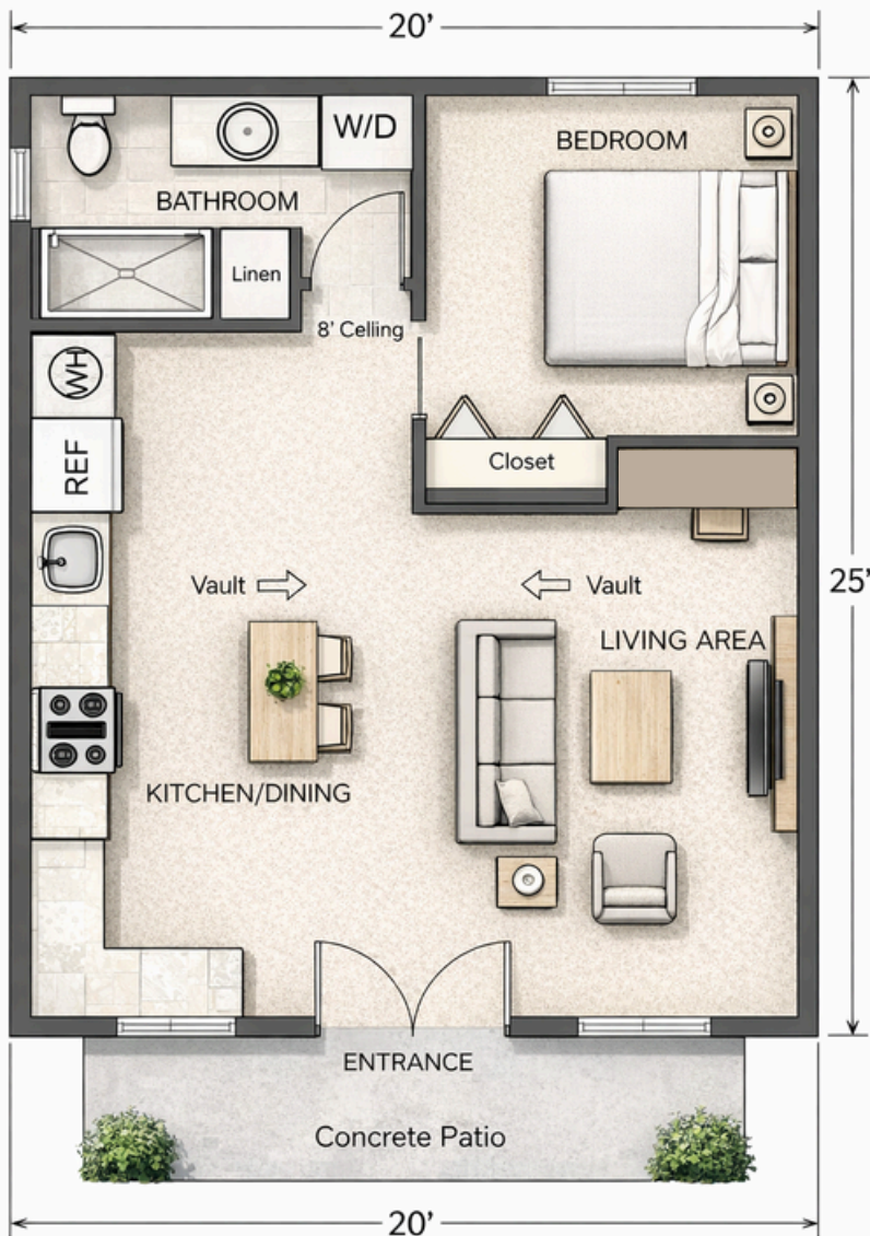
Haven – Gable Side Entry 20' x 25' - 500 sq. ft.
